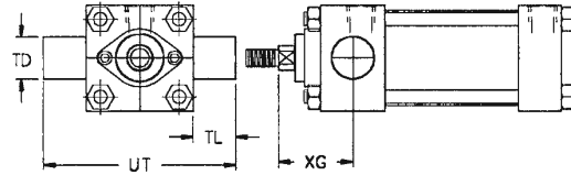
Mount Code T6 (Removable Aluminum Trunnion Ears)
