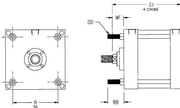
Mount Code X3
