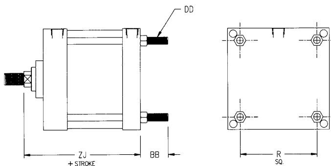
Mount Code X2
