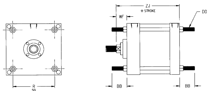
Mount Code X1
