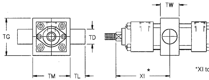
Mount Code T8 (Removable Trunnion Ears)
